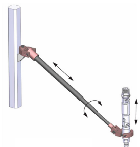
Vertical tightening axis
