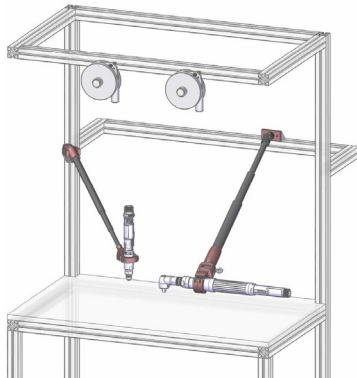
Vertical tightening axis
