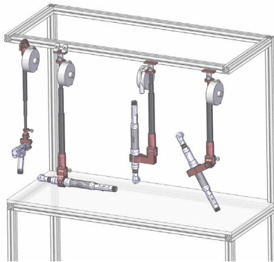
Horizontal tightening axis
